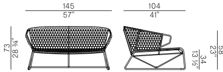
698/D divano \ sofa cuscino \ cushion
