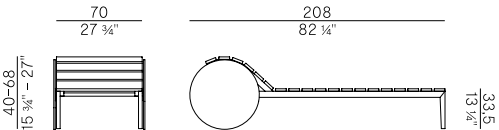
895/D-RECL lettino \ sunbed
