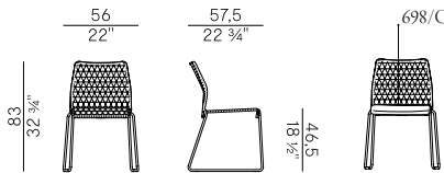
698 sedia dining impilabile \ stackable dining chair ×6 cuscino \ cushion
