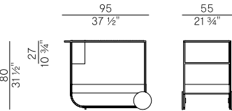
892 carrello \ trolley
