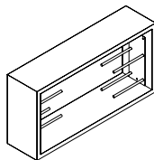
Rettangolo Bottle design: Ronda Design Lab L 600 H 300 P 150 mm
