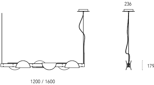
Dimensioni - Dimensions (mm) Sundown Moon
