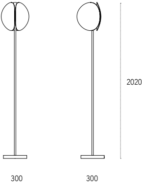
Dimensioni - Dimensions (mm) Flake Floor
