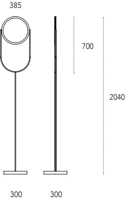
Dimensioni - Dimensions (mm) Lift Floor
