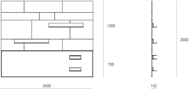
Dimensioni - Dimensions (mm) Caddy + Magnetic backsplash
