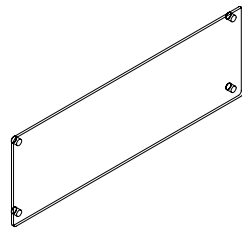
Parafiamma Baffle plate design: Ronda Design Lab L 900 H 300 P 29 mm
