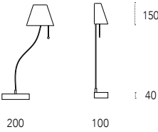
Dimensioni - Dimensions (mm) Lapilla
