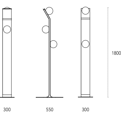
Dimensioni - Dimensions (mm) Brand Floor
