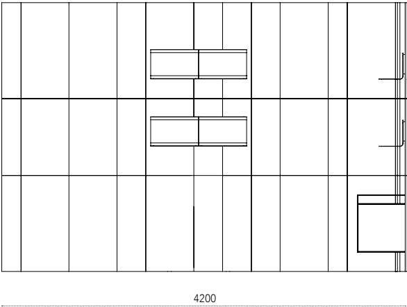
Dimensioni - Dimensions (mm) Caddy home office - side A
